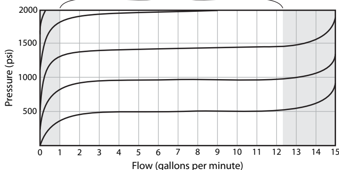
BR 10 recommended operating range
