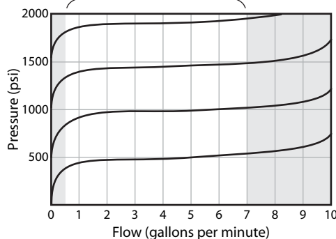
BR 5 recommended operating range
